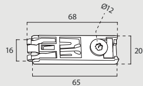
LOCK *mm
